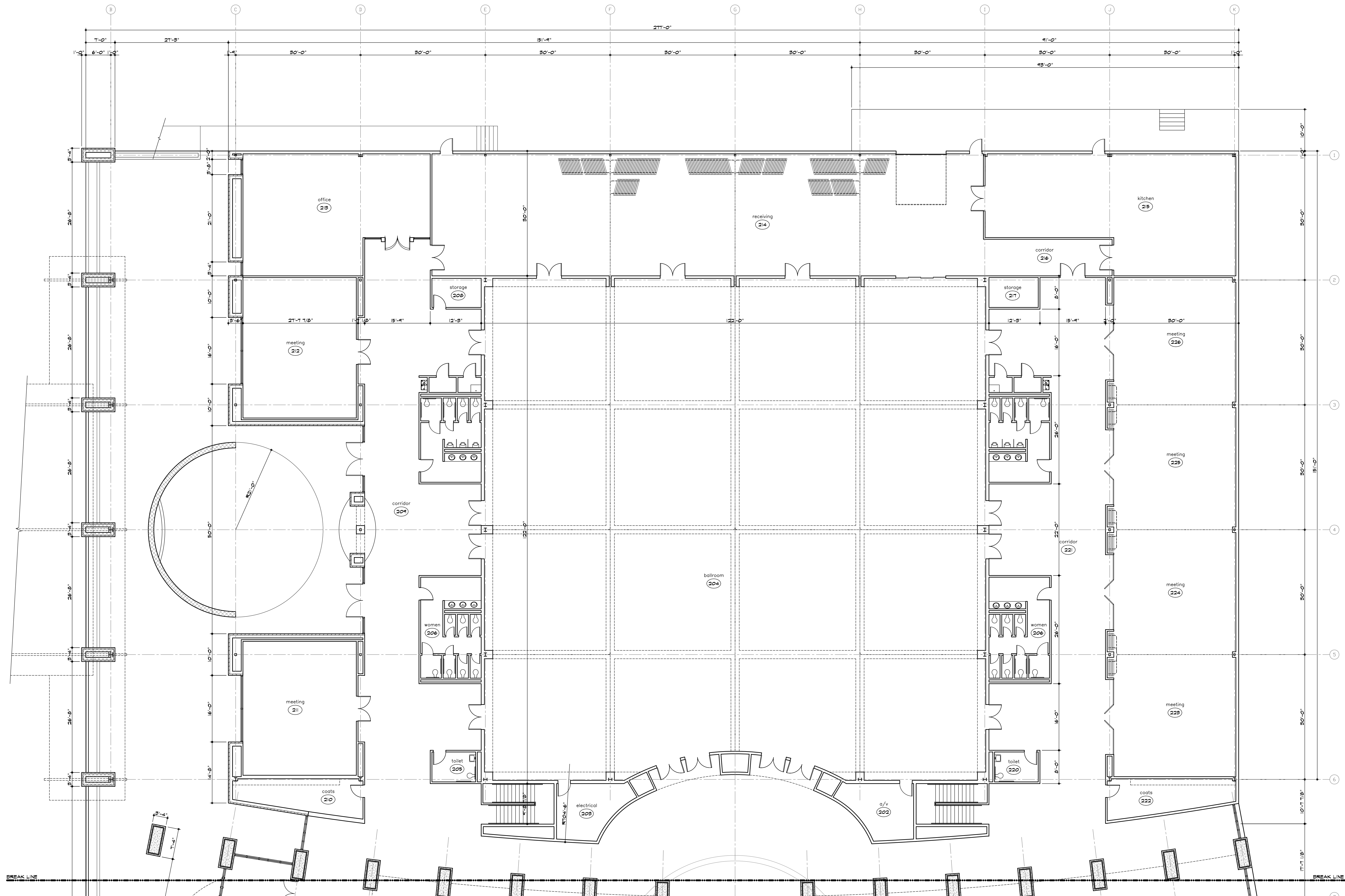
1 MAIN LEVEL FLOOR PLAN - BALLROOM SCALE: 1/8" = 1'-0"
